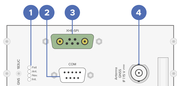
Two slot IMS-XHE Rb Connector and COM Model
